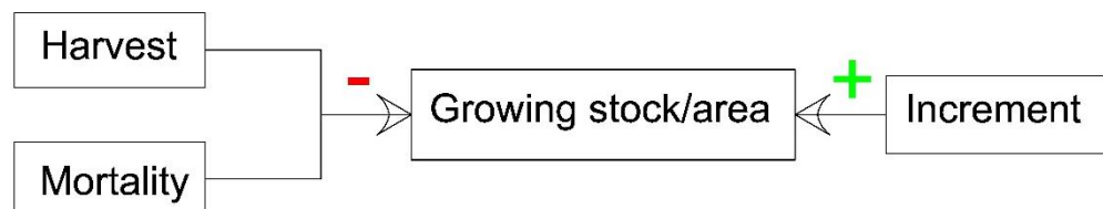
Figure 1: Growth Flowchart
